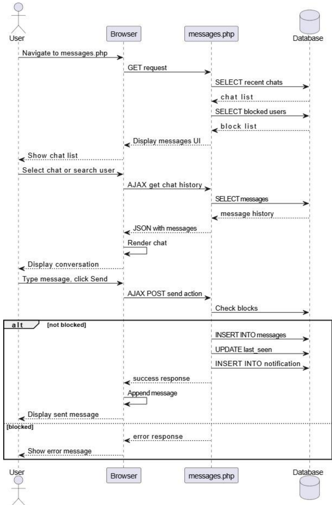
Figure 4-8 Sequence Diagram of Direct Messaging
