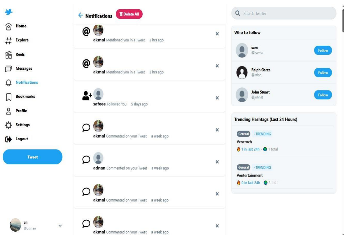
Figure 6-9 Notifications Page
