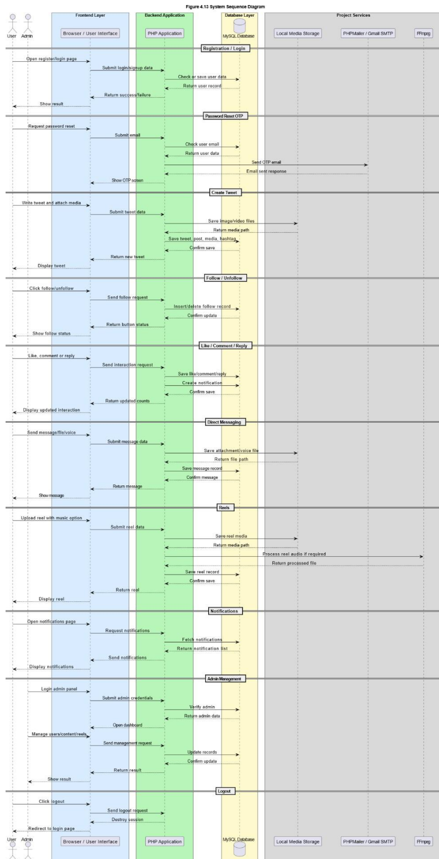
Figure 4-13 System Sequence Diagram
