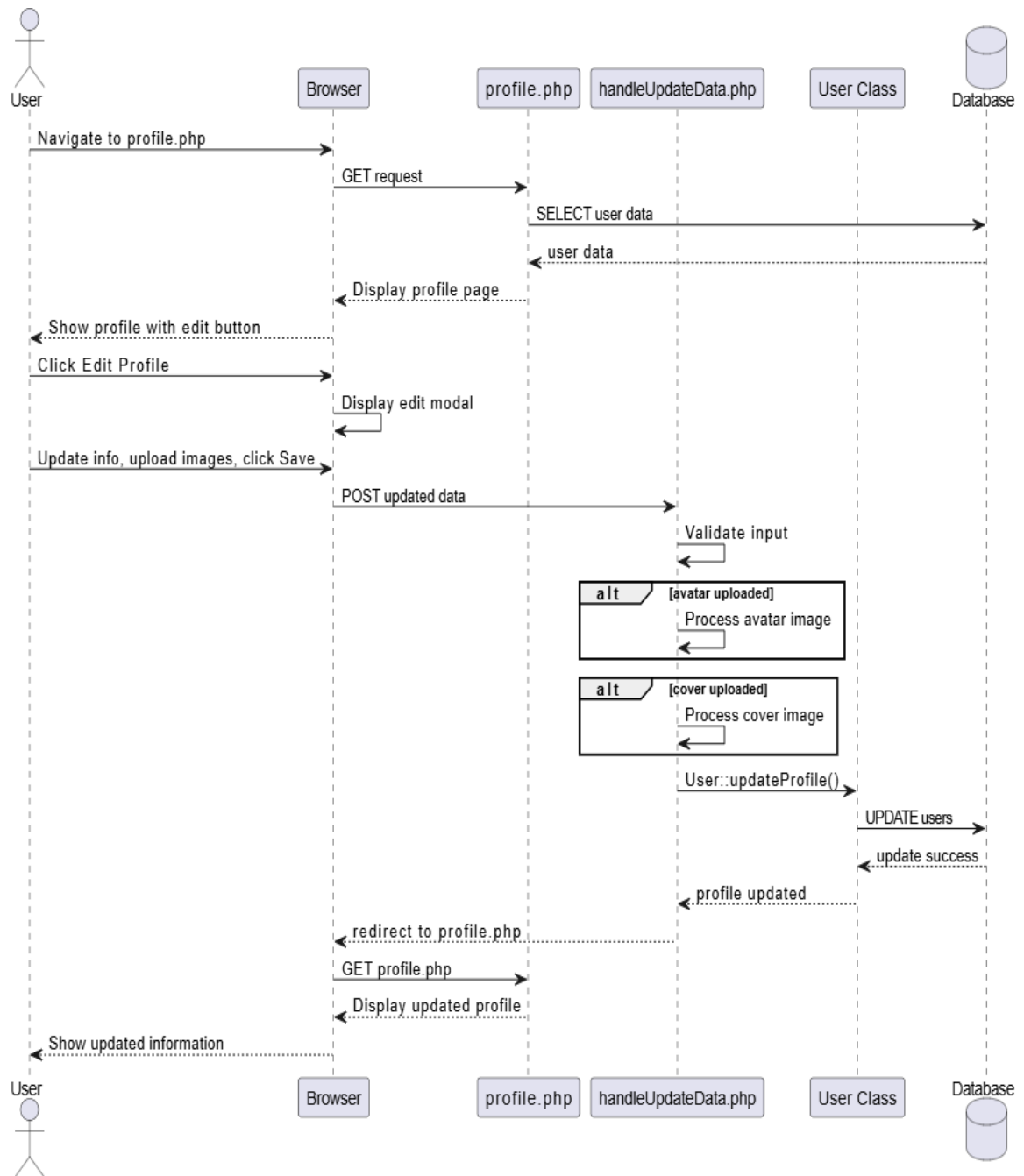
Figure 4-5 Sequence Diagram of View and Update Profile
