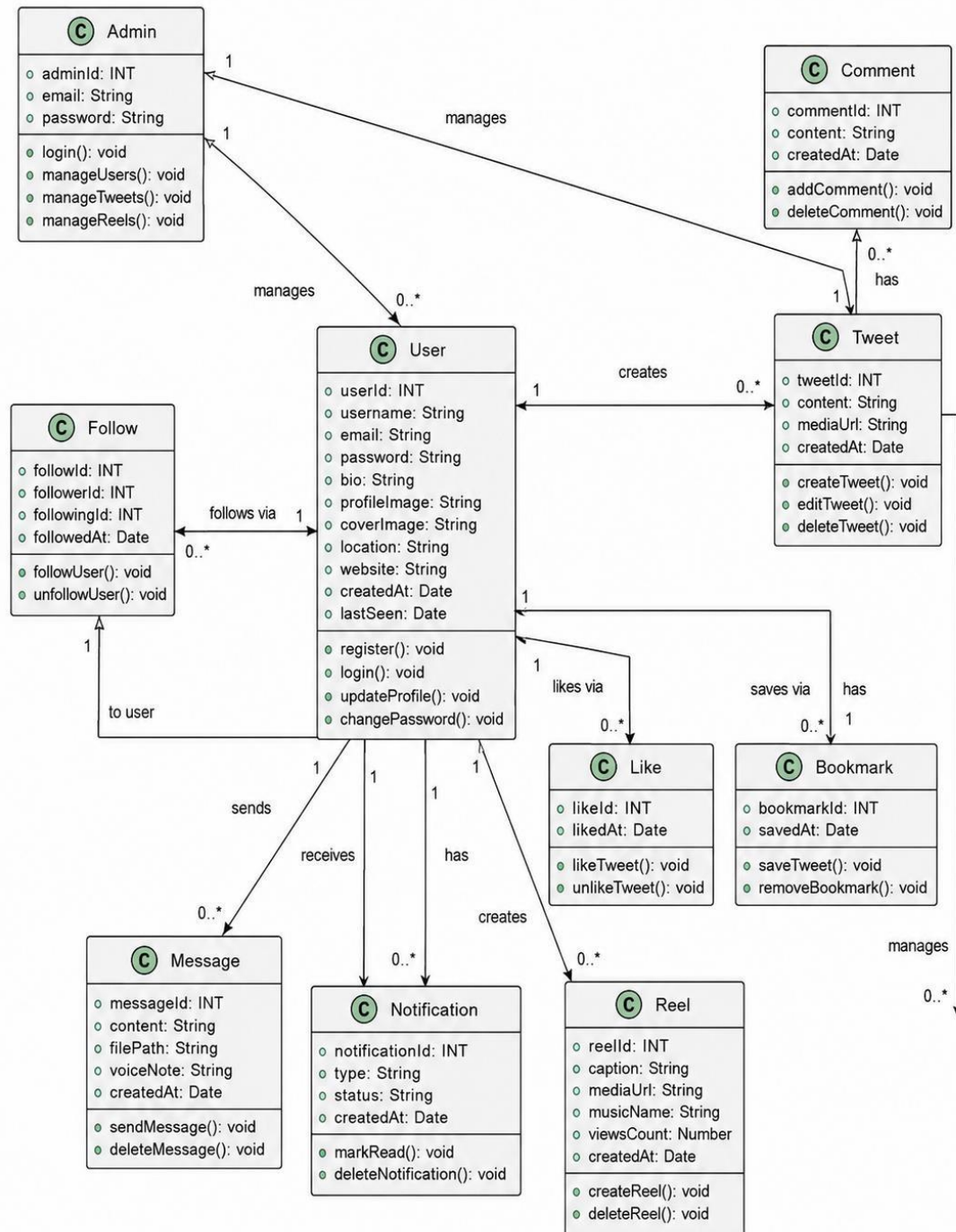
Figure 4-14 Class Diagram
