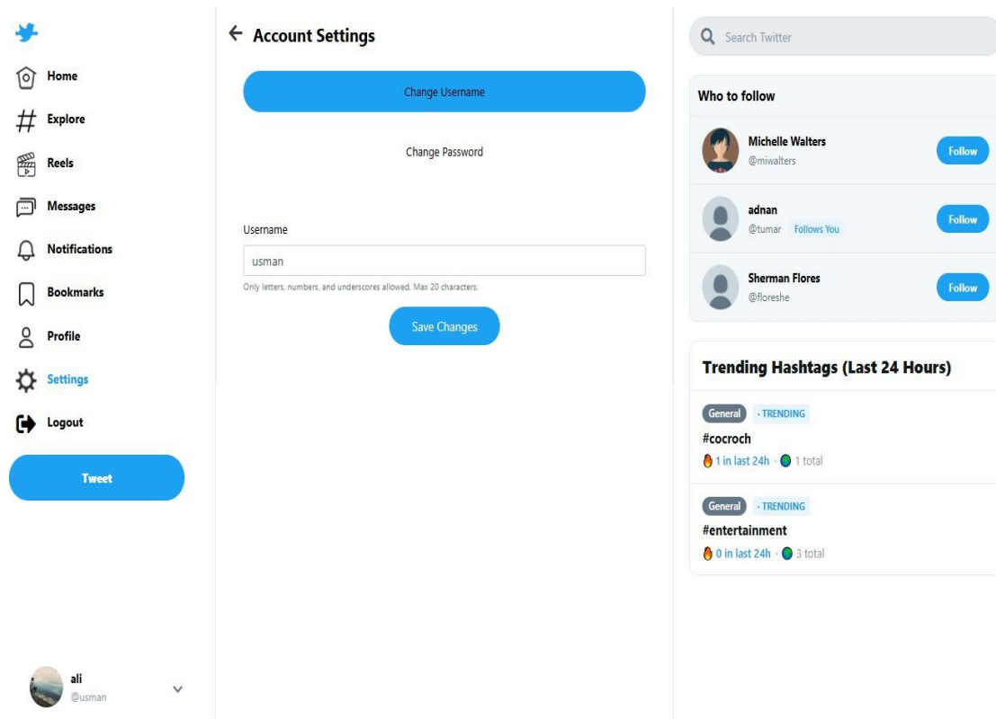
Figure 6-11Account Settings Page
