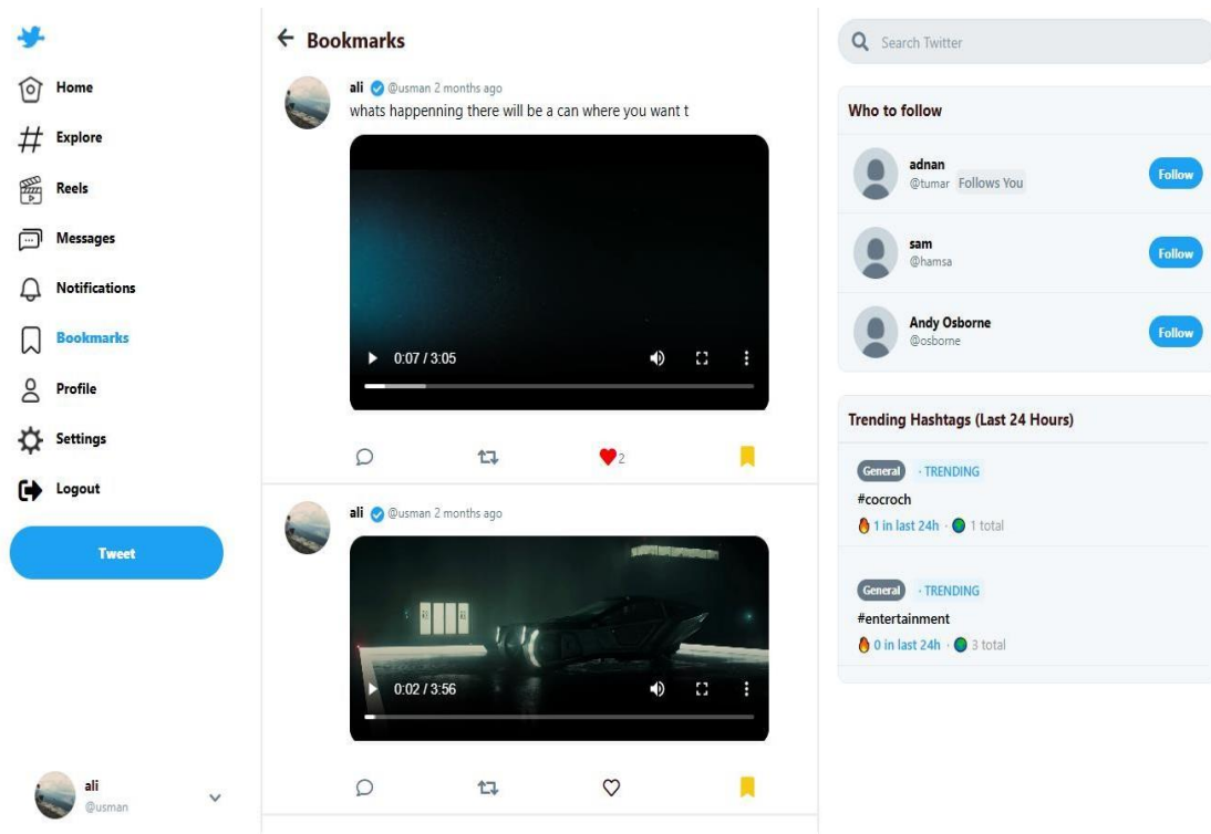
Figure 6-8 Bookmarks Page
