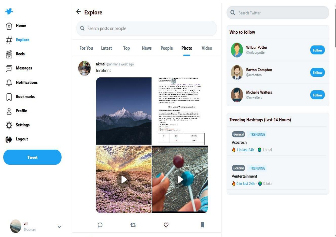
Figure 6-5 Explore Page
