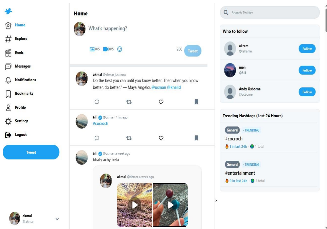
Figure 6-3Home Page Dashboard
