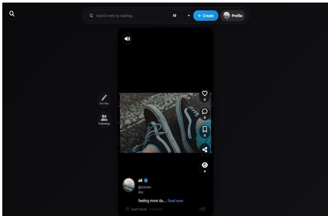
Figure 6-6 Reels Page
